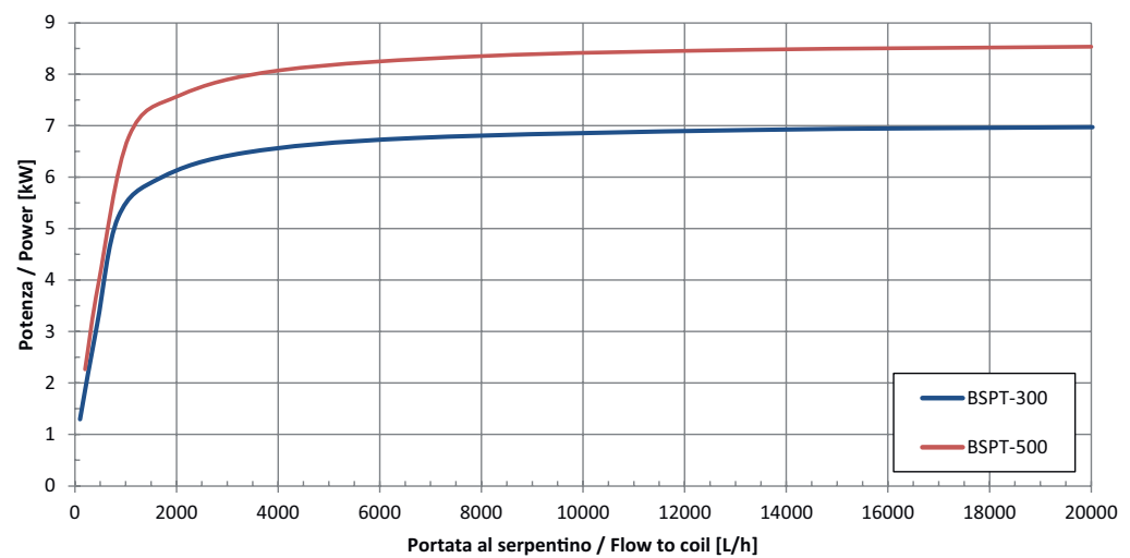
Potenza scambiata, scamb.integr. T_{in,coil} = 60\text{ °C} ; T_{serb,in} = 10\text{ °C} , T_{serb,out} = 45\text{ °C}
