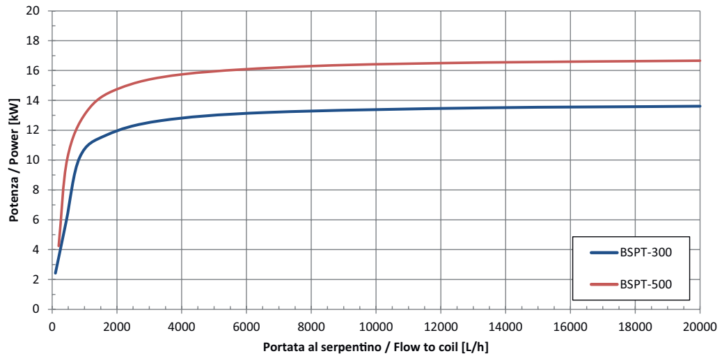
Potenza scambiata, scamb.integr. T_{in,coil} = 80\text{ °C} ; T_{serb,in} = 10\text{ °C} , T_{serb,out} = 45\text{ °C}
