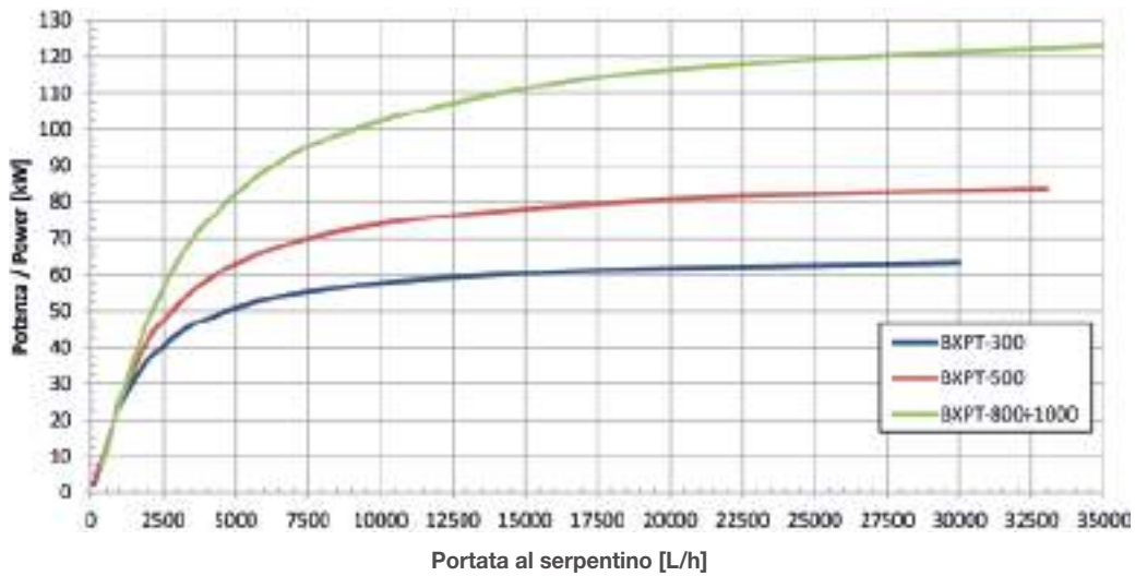
Potenza scambiata, scamb. PdC T_{in,coil} = 50\text{ °C}; T_{serb,in} = 10\text{ °C}, T_{serb,out} = 45\text{ °C}
