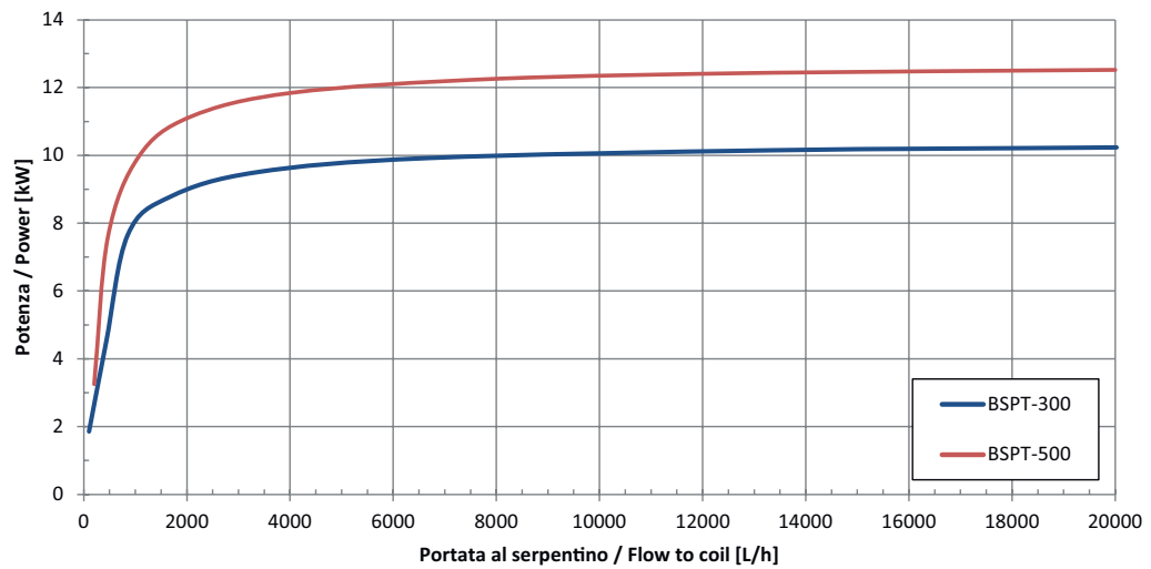
Potenza scambiata, scamb.integr. T_{in,coil} = 70\text{ °C} ; T_{serb,in} = 10\text{ °C} , T_{serb,out} = 45\text{ °C}
