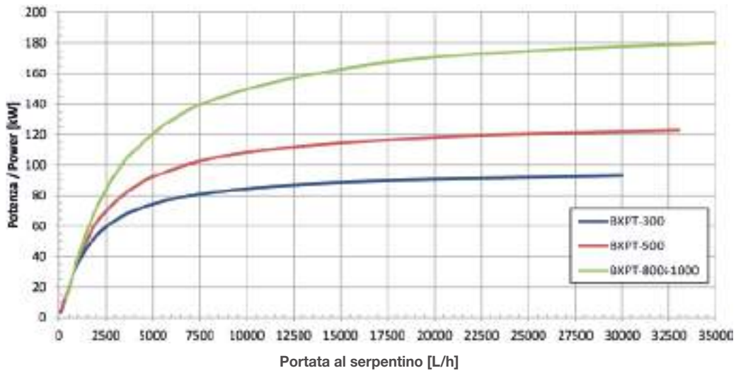
Potenza scambiata, scamb. PdC T_{in,coil} = 60\text{ °C}; T_{serb,in} = 10\text{ °C}, T_{serb,out} = 45\text{ °C}
