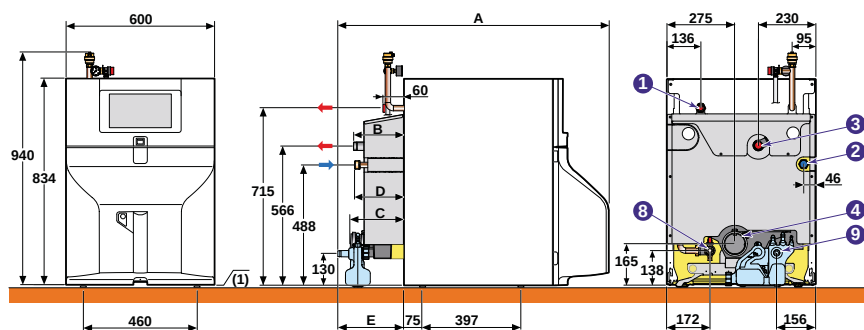
Power HT OIL 24 e 32
